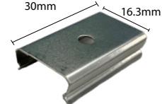
Support de montage (Flexitube RGB)
