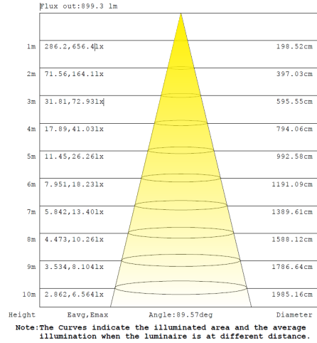
Illuminance at distance
