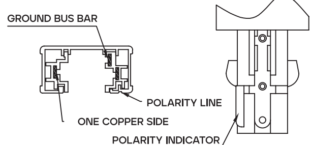
FIG. 2 STANDARD POLARITY
